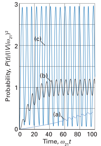
Fig. 6.17 The time variation of the probability of occupying an initially unoccupied state when the perturbation is switched on at different rates; the different values of the switching rate are expressed by the parameter \lambda = k/\omega_{21} with (a) \lambda = 0.01 , (b) \lambda = 0.1 , (c) \lambda = 1 .
