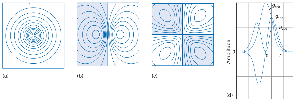
Fig. 9.2 Gaussian orbitals. (a), (b), and (c) show the contour plots for s-, p-, and d-type Gaussians, respectively, with the form e^{-r^2} , xe^{-r^2} and xye^{-r^2} . (d) Cross-sections through the three functions.
