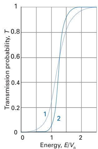
Fig. 2.17 The transmission probability for an Eckart barrier and its variation with energy. The curves are labelled with the value of (2mV_0)^{1/2}/\beta\hbar .
