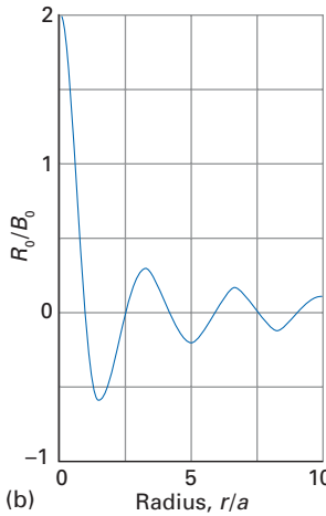
Fig. 14.9 (a) The function u_0(r) and (b) the accompanying radial wavefunction R_0(r) for S-wave scattering by a spherical square well. The illustration is based on a(2\mu V_0)^{1/2}/\hbar = 3 and E/V_0 = 0.4 .
