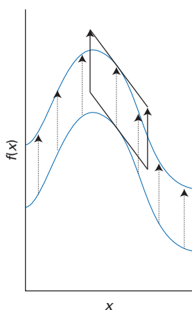
Fig. 13.4 A constant can be added to a function without changing the latter's slope. The generalization of this feature is a gauge transformation of A , a modification of A that leaves B unchanged.
