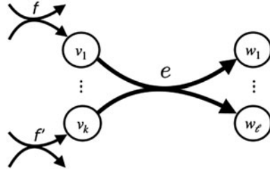
FIG. 1. A generic hyperedge e with \text{tail}(e) = \{v_1, \dots, v_k\} and \text{head}(e) = \{w_1, \dots, w_\ell\} . In general, to use e in a hyperpath P , for every vertex v \in \text{tail}(e) there must be a hyperedge f that precedes e in P with v \in \text{head}(f) .
