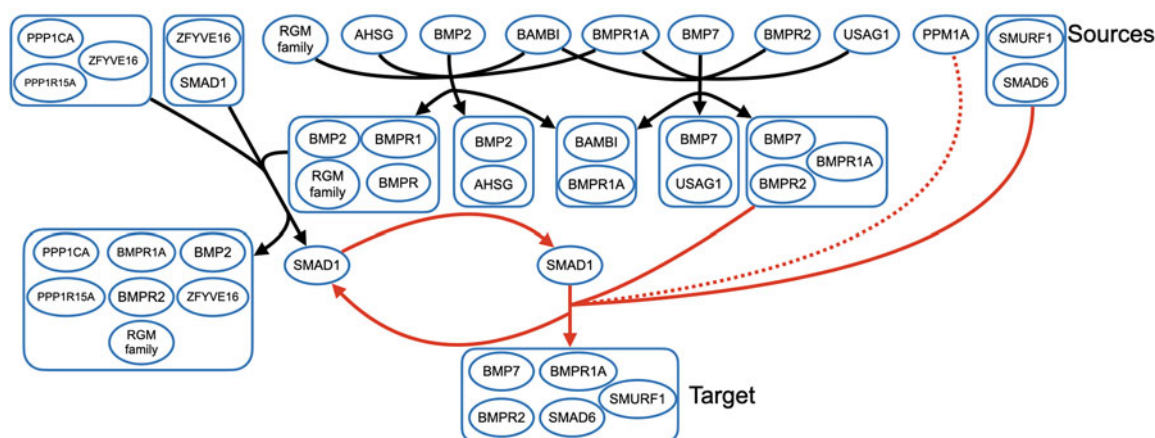
FIG. 4. Shortest hyperpath to the BMP7/BMPR2/BMPR1A/SMAD6/SMURF1 complex. Sources are shown across the top of the figure, and the target is shown at the bottom. The portion of the final hyperedge in dotted red represents PPM1A acting as a positive regulator of the reaction. The hyperedges in red form a cycle in the hyperpath.
