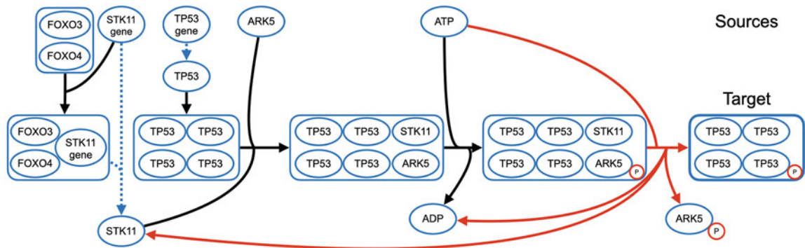
FIG. 3. Shortest hyperpath to the phosphorylated p53 tetramer. Sources are shown across the top of the figure, and the target is in the bottom right corner. The hyperedges in dotted blue represent transcription/translation events. The hyperedge in red creates a cycle in the hyperpath, as node STK11 in its head occurs in the tail of a prior hyperedge in the hyperpath.
